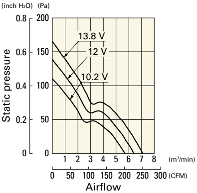
109E1712H501 With pulse sensor
